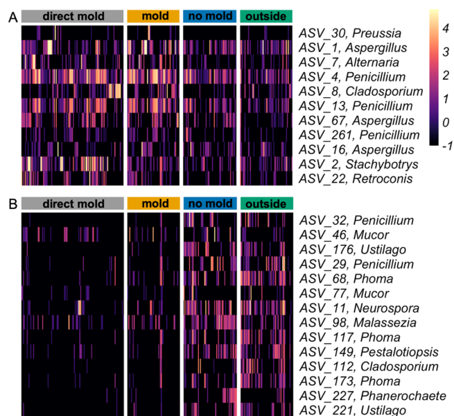
Figure 2. Heatmap of the statistically significant \log_2 fold ( \log_2 F ) changes between mold and no mold indoor air-settled dust ( p_{\text{adj}} \leq 0.01 ): (A) ASVs that were more abundant among the mold samples than the no mold samples and (B) ASVs that were more abundant among the no mold samples than the mold samples. Heatmap is colored by the \log_{10} relative abundances with the most highly abundant taxa in yellow and those taxa not present in a sample in black.
