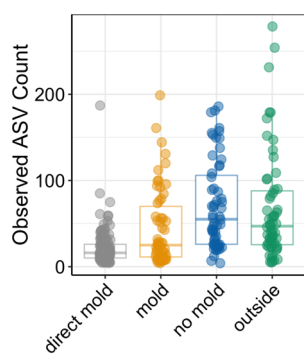
Figure 1. Fungal richness scatterplot based on ASV count. Boxplots (25th quartile, median, 75th quartile) are overlaid with each scatterplot. Samples are colored by their sample type: direct mold—grey, mold—orange, no mold—blue, and outside—green.
